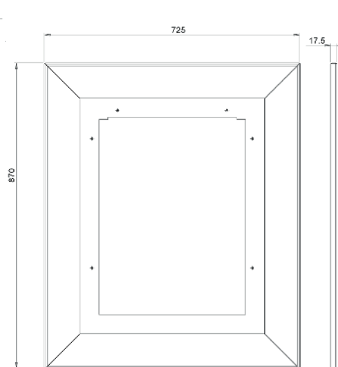
4 sided backplate
