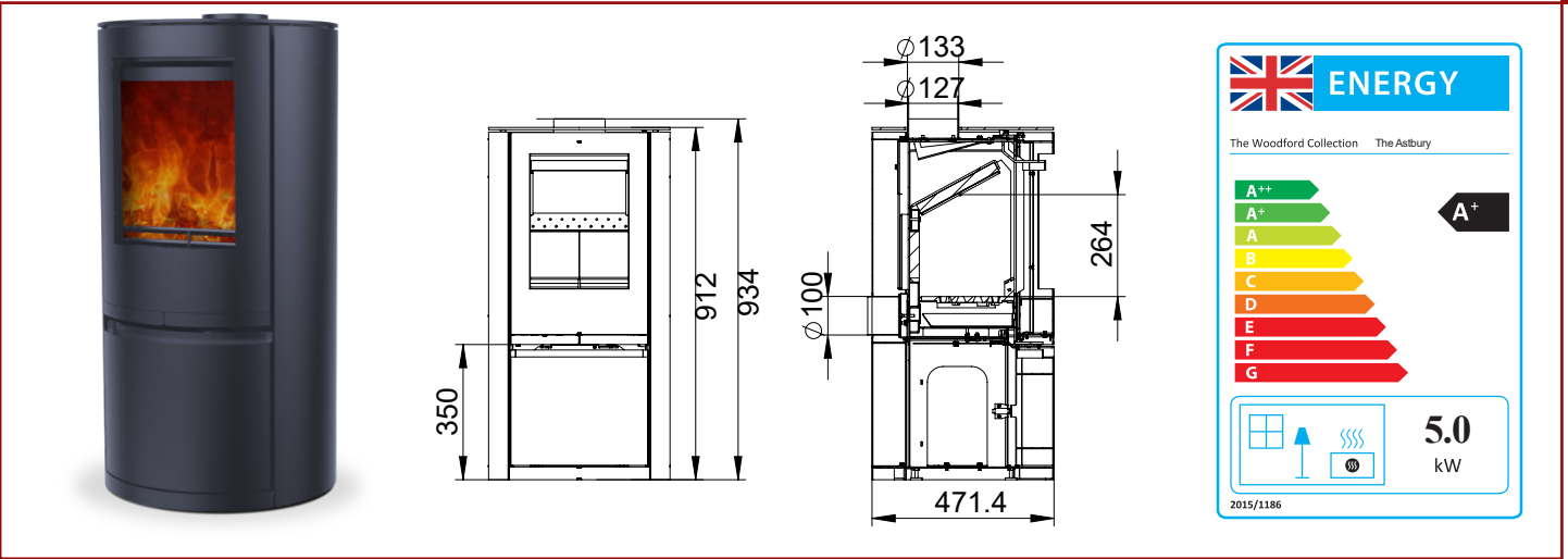
THE ASTBURY Distance to combustibles: 500mm Top, 50mm Side, 50mm Rear
